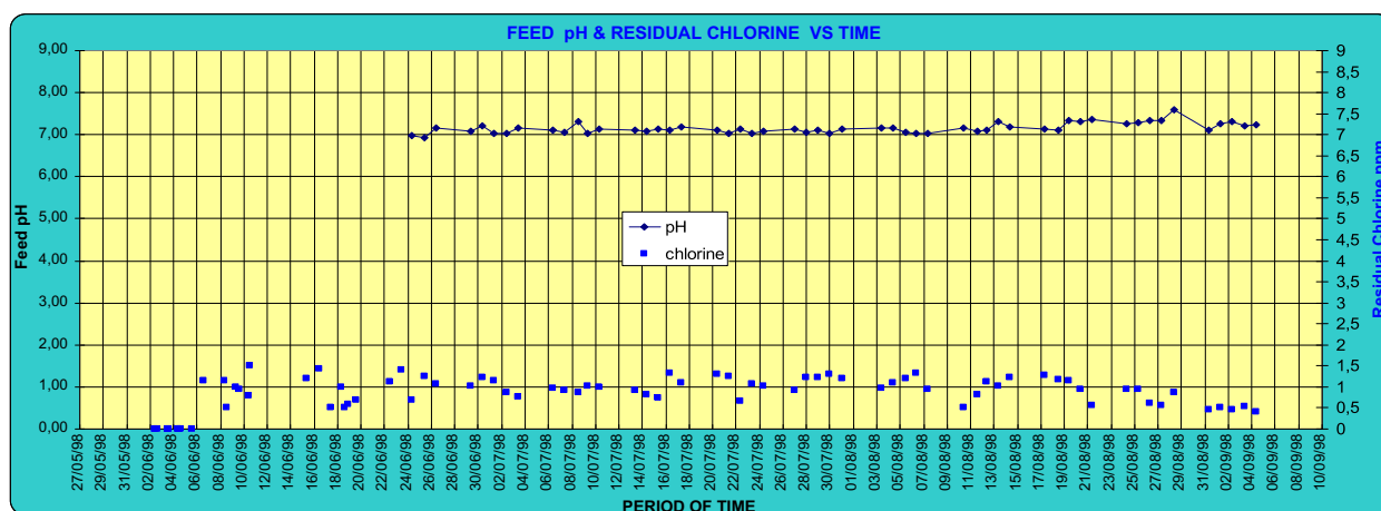
Fig. 1. Analysis of test data: Toyobo pilot plant (Stage 1).
