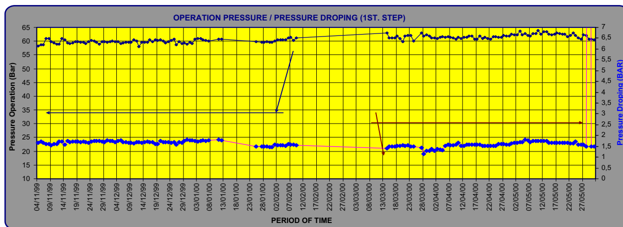
Fig. 15. Membrane performance: stage 3.
