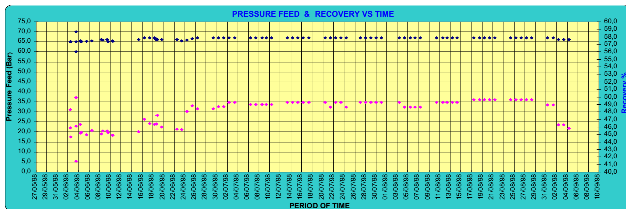
Fig. 3. Analysis of test data: Toyobo pilot plant (Stage 1).
