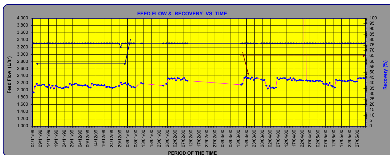
Fig. 14. Membrane performance: stage 3.
