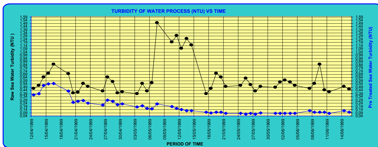
Fig. 10. Analysis of test data: EM pilot plant (Stage 1 and 2).
