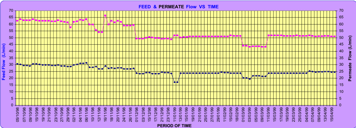
Fig. 6. Analysis of test data: Toyobo pilot plant (Stage 2).
