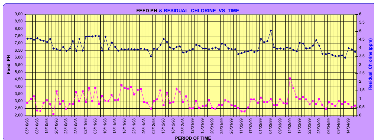
Fig. 5. Analysis of test data: Toyobo pilot plant (Stage 2).
