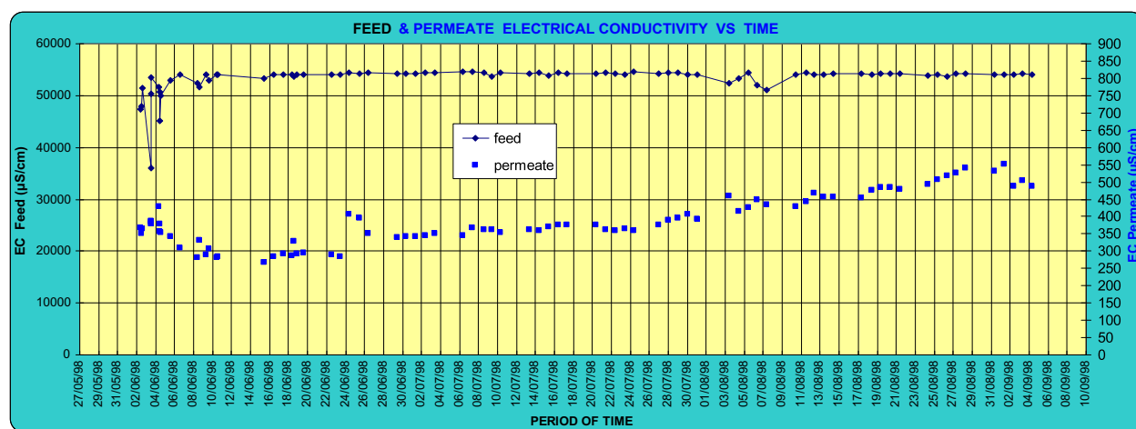
Fig. 4. Analysis of test data: Toyobo pilot plant (Stage 1).
