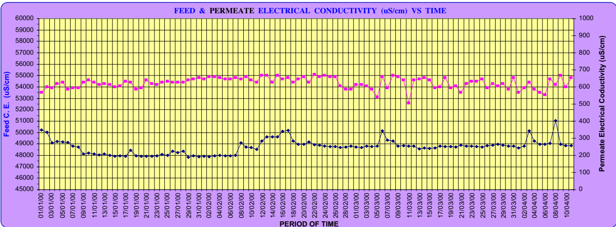
Fig. 8. Analysis of test data: Toyobo pilot plant (Stage 2).
