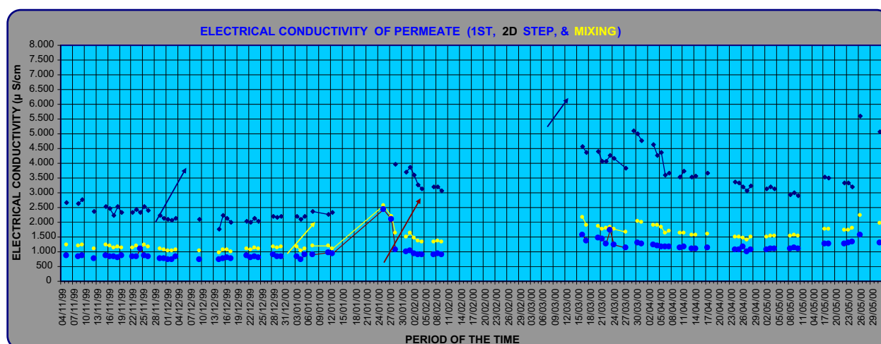
Fig. 17. Membrane performance: stage 3.
