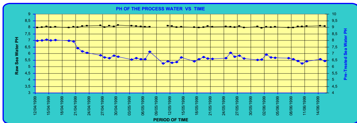
Fig. 9. Analysis of test data: EM pilot plant (Stage 1 and 2).
