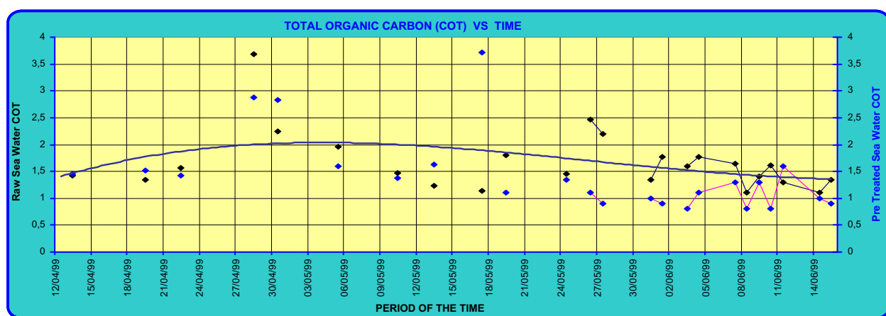
Fig. 12. Analysis of test data: EM pilot plant (Stage 1 and 2).
