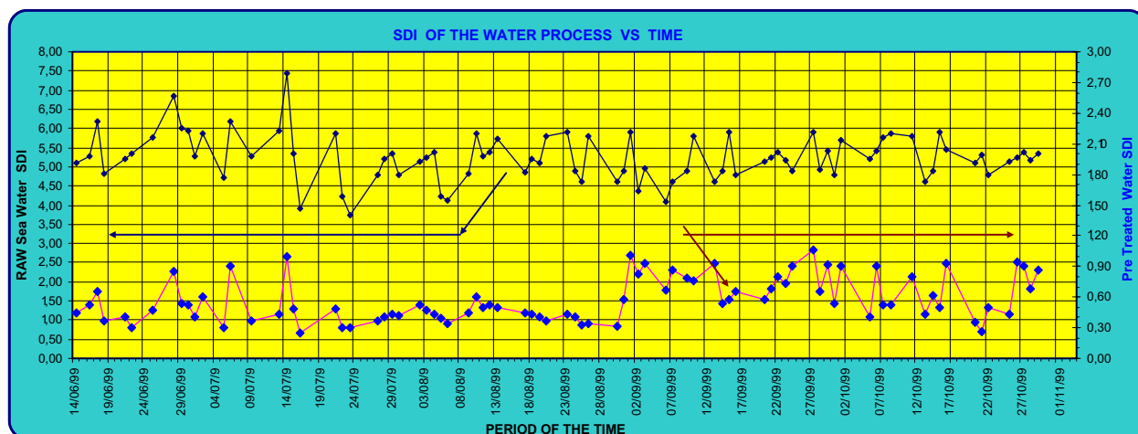
Fig. 11. Analysis of test data: EM pilot plant (Stage 1 and 2).
