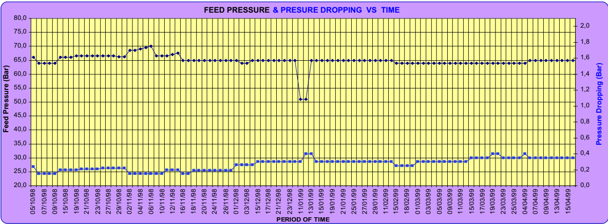
Fig. 7. Analysis of test data: Toyobo pilot plant (Stage 2).
