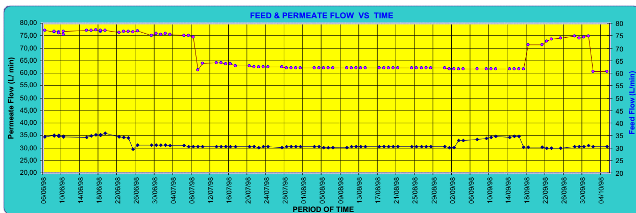
Fig. 2. Analysis of test data: Toyobo pilot plant (Stage 1).
